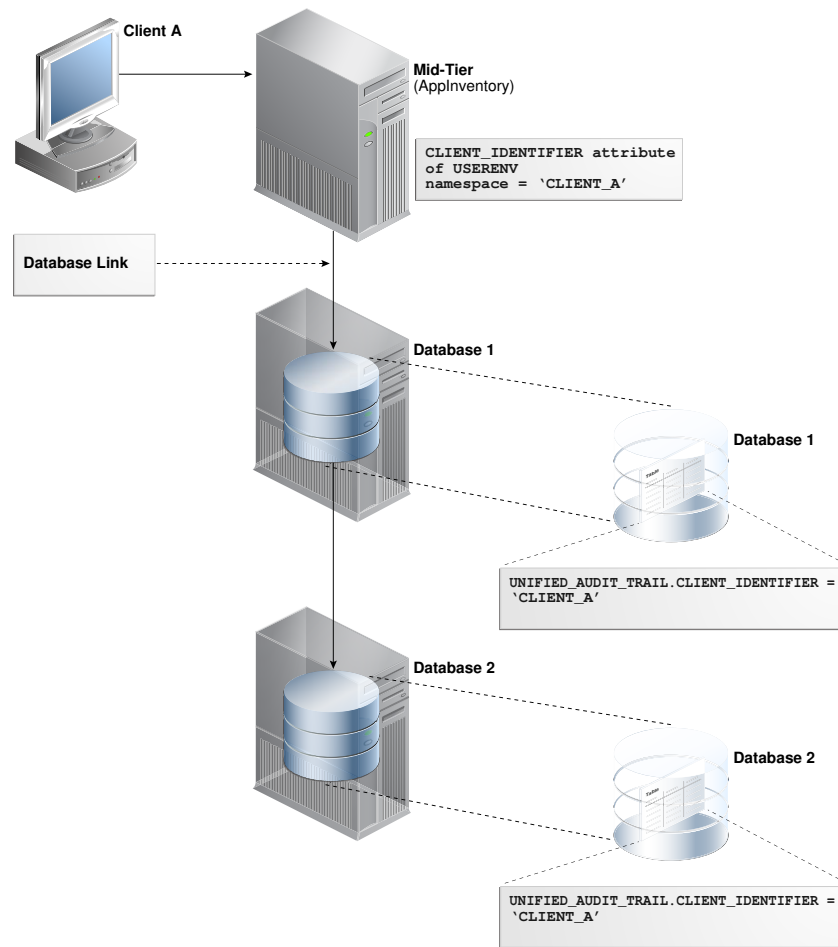
Figure 24-2 Auditing Client Identifier Information Across Sessions
