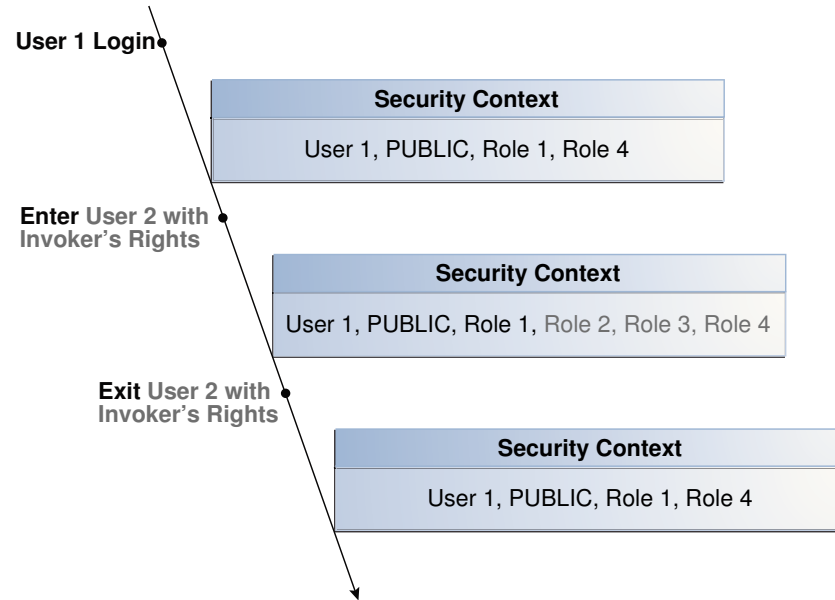
Figure 6-2 Security Context in Which Invoker's Right Program Unit IR Is Executed
