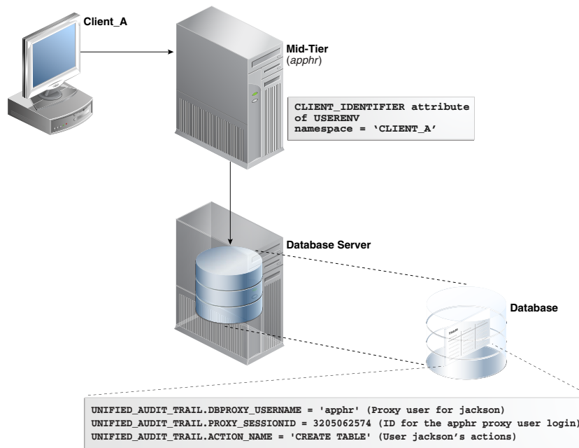
Figure 24-1 Auditing Proxy Users
